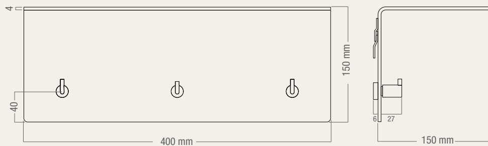
COAT RACK 4004
