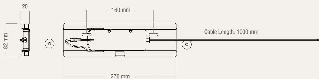
BACKLIGHT BAR 4000-400
