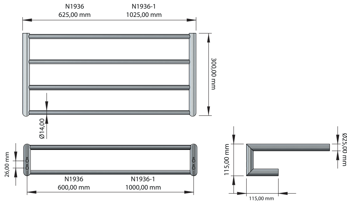
WARDROBE SHELF 1 & 2
